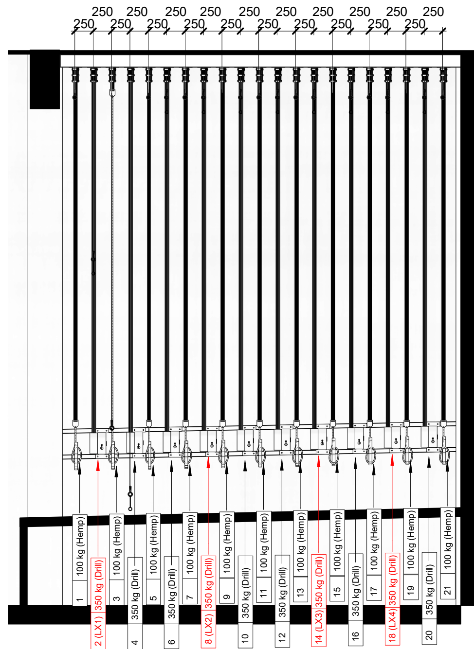
Stagehouse - Long Section
