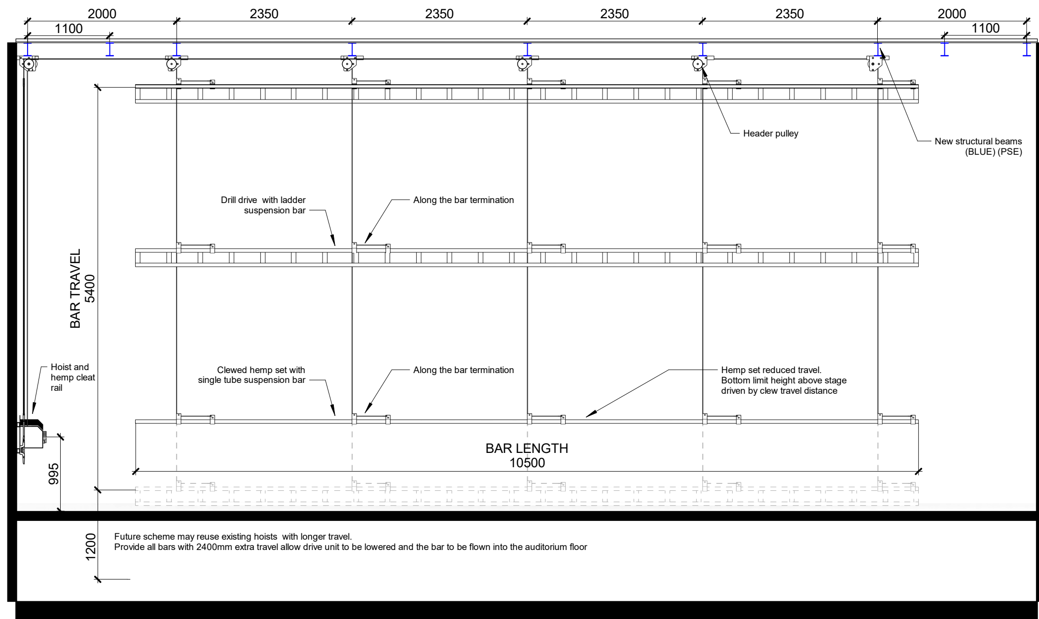
Stagehouse - Cross Section
