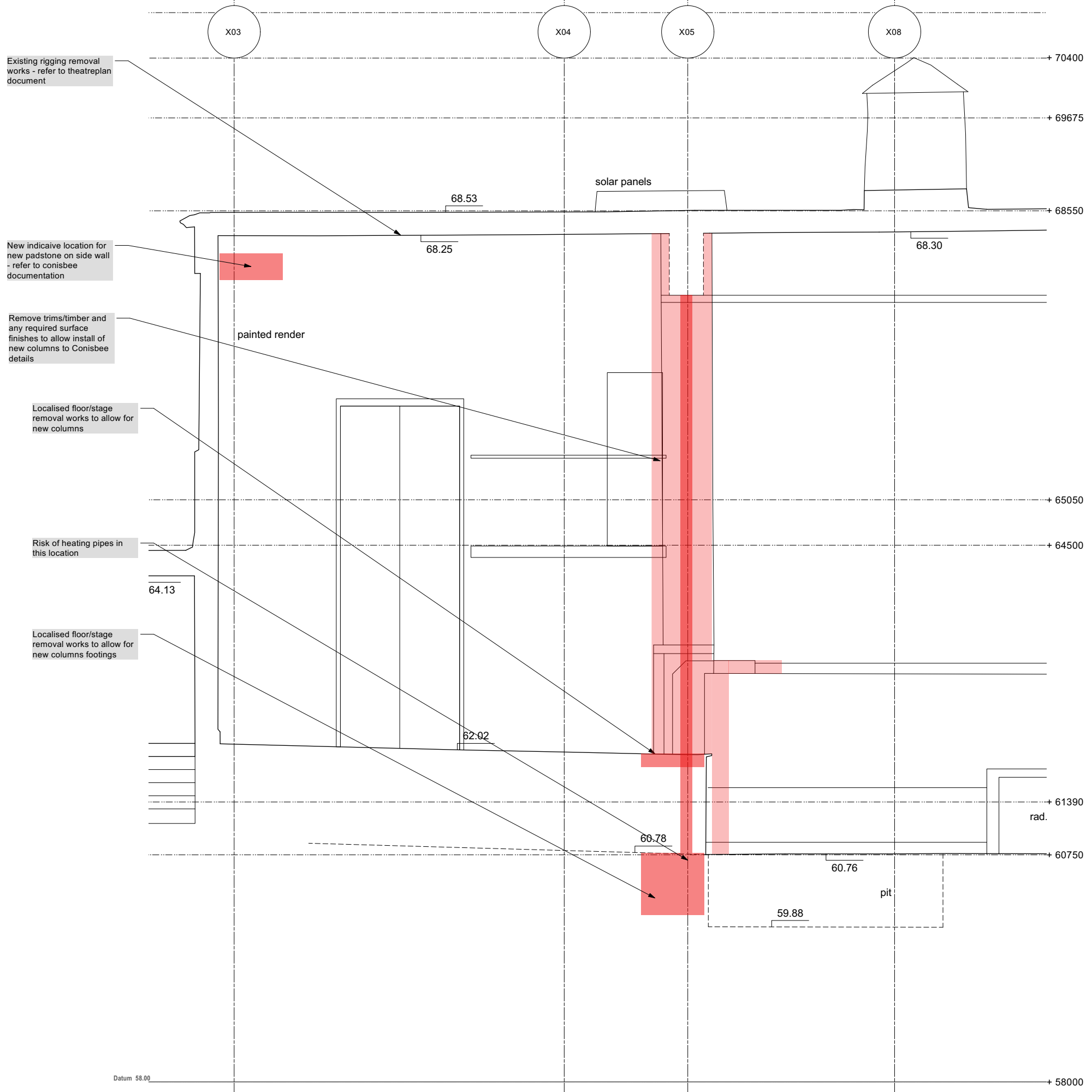
SECTION CC 1:25@A1
